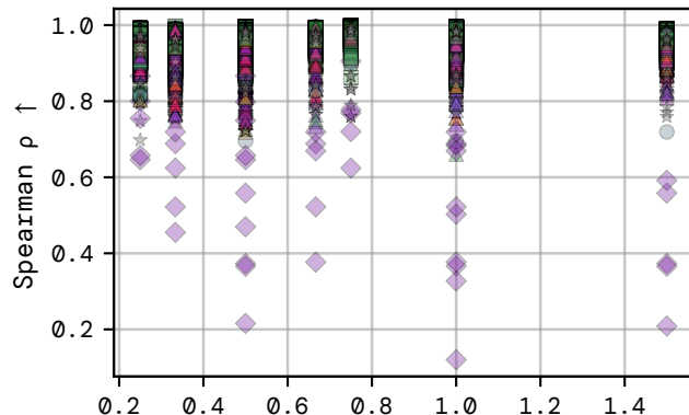
Spearman \rho
