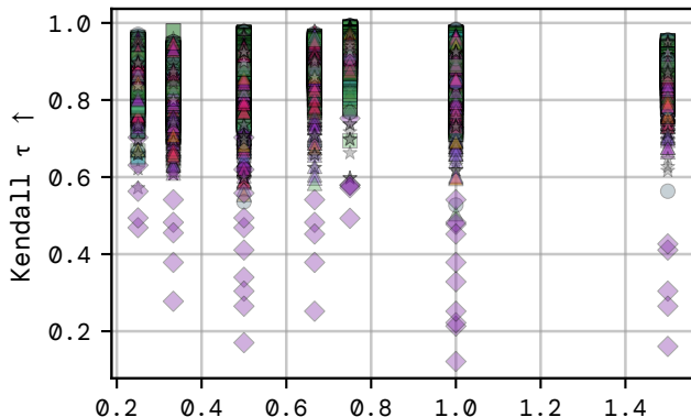
Kendall \tau
