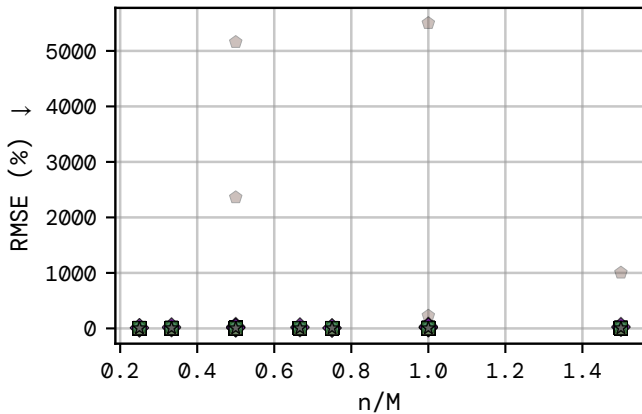
Kendall \tau
